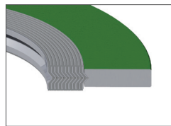
Winding w/ Centering Ring
