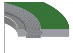
Winding w/ Inner & Centering Ring
